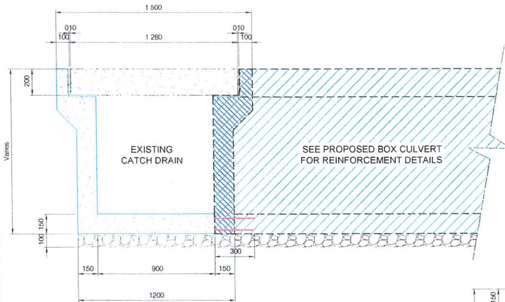
PART OF LONGITUDINAL SECTION ELEVATION
