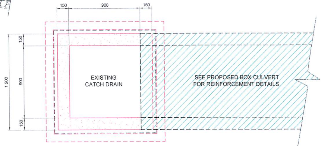
GROUND PLAN
