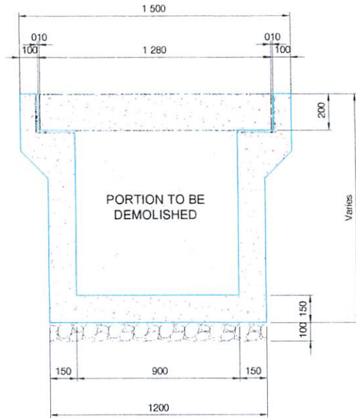
SECTION
