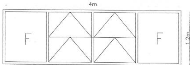
(W8) 1 SET ( 4m x 1.2m) W/6MM THK GLASS
